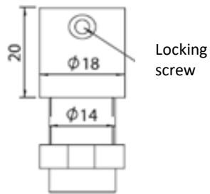
Floor tightener
