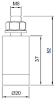
Façade tightener
