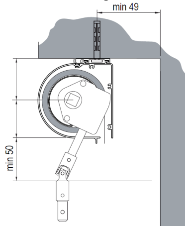
Internal ceiling installation
