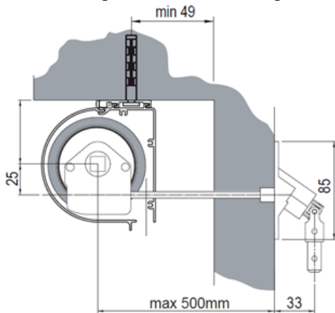
External ceiling installation with wall grommet
